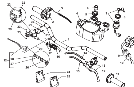
TAV.15 Comandi-Manubrio - Controls-Handlebars - Commandes-Guidon - Bedienungselemente-Lenker - Mandos-Manillar
