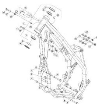
TAV.31 Telaio - Frame - Chassis - Rahmen - Chasis
